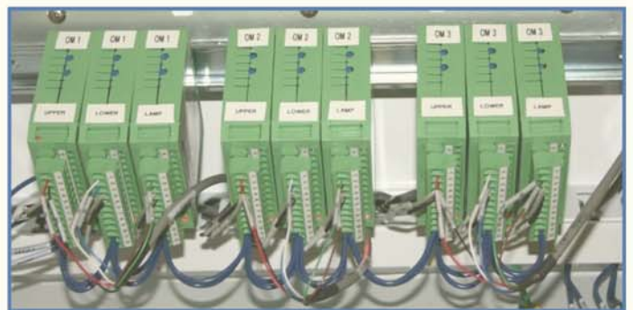
EIT DIN Rail units installed in cabinet to support multiple Compact Sensors used in production.
