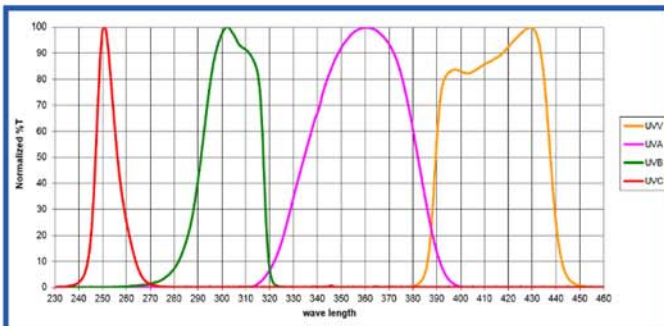
EIT Mercury (Broadband) Responses: UVC, UVB, UVA, UVV *The Compact Sensor UVC Response is 240-260 nm
