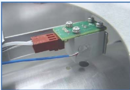
An EIT Compact Sensor mounted behind a UV reflector can provide continuous information on the lamp condition.
